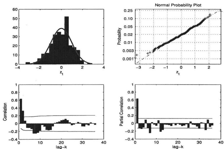
Figure 2. Data Plot.
