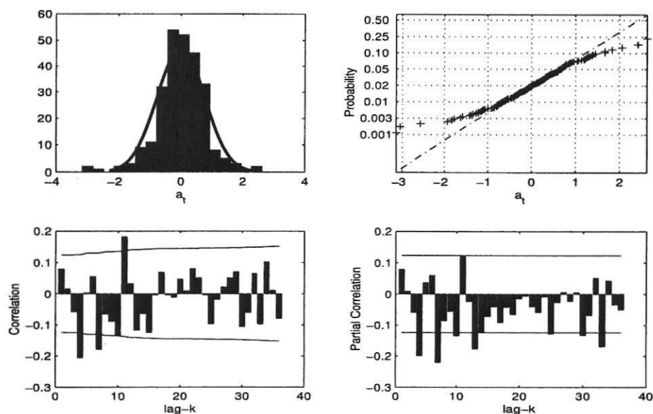
Figure 3. Residual Analysis.
