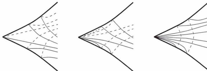
Figure 15: Regions with two separatrices.
