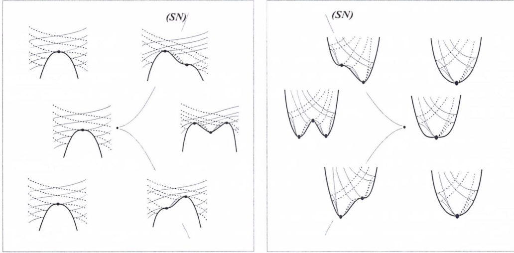
Figure 3: Bifurcations of p^2 + (-y + \epsilon x^4 + ux + vx^2) = 0 , \epsilon = -1 left and \epsilon = +1 right.
