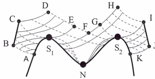
Figure 2: A neighbourhood of the discriminant.
