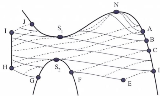
Figure 5: A neighbourhood of the discriminant.
