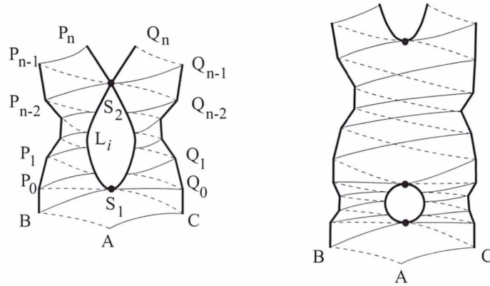
Figure 7: Neighbourhood of the discriminant.
