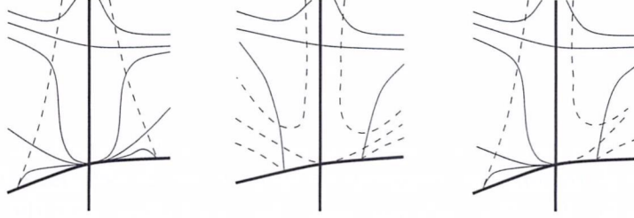
Figure 10: The case l > 2k .
