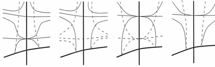
Figure 11: The case l = 2k .
