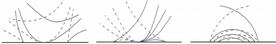
Figure 1: Well-folded saddle (left), node (centre) and focus (right).
