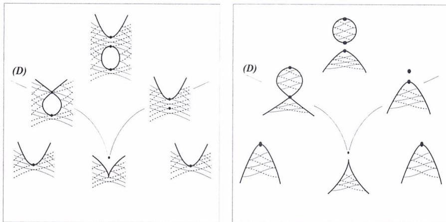
Figure 6: Bifurcations of p^2 + (\epsilon x^2 + y^3 + uy + v) = 0 , \epsilon = -1 left and \epsilon = +1 right.
