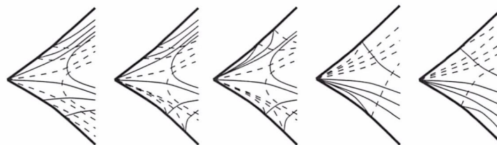
Figure 16: Regions with four separatrices.
