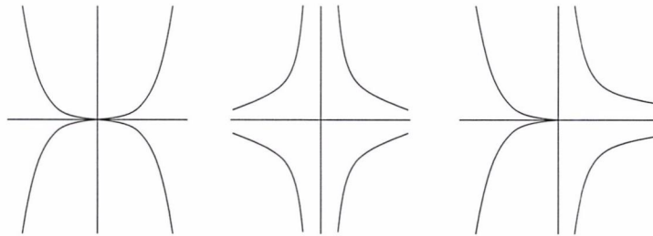
Figure 9: Integral curves of tdx \pm x^{l-2k}dt = 0 .
