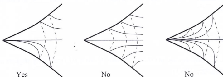
Figure 14: Regions with one separatrix.
