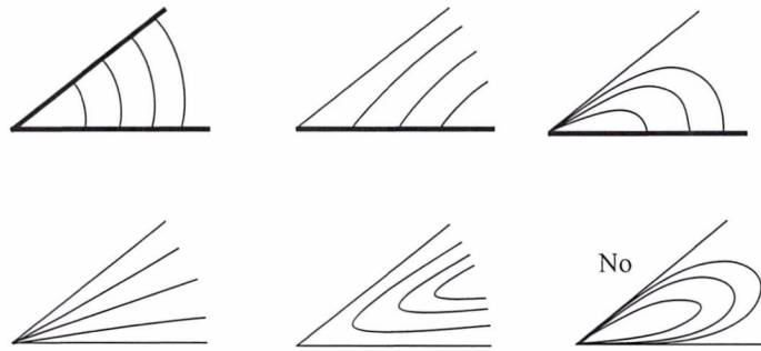
Figure 12: The possible sector configurations for one directional field.
