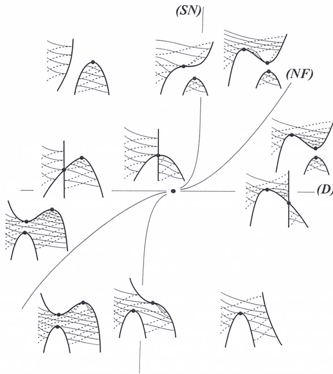
Figure 4: Bifurcations of p^2 + (xy + x^3 + ux^2 + v) = 0 .
