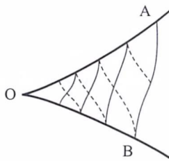
Figure 13: Region without a separatrix.
