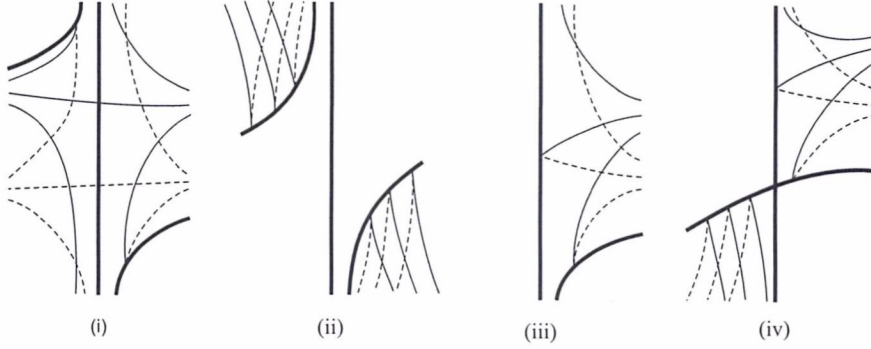
Figure 8: The case l < 2k , l even (i) and (ii), l odd (iii) and (iv).
