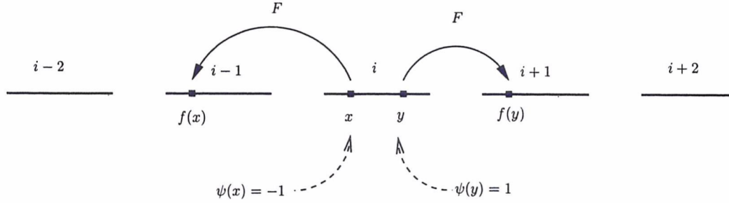
FIG. 1. A deterministic random walk
