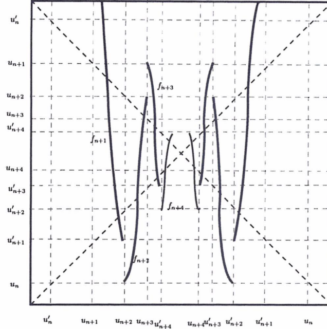
FIG. 5. Induced map F for a Fibonacci map
