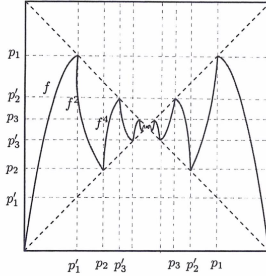
FIG. 2. The "Bat" map: the induced map F for a Feigenbaum unimodal map
