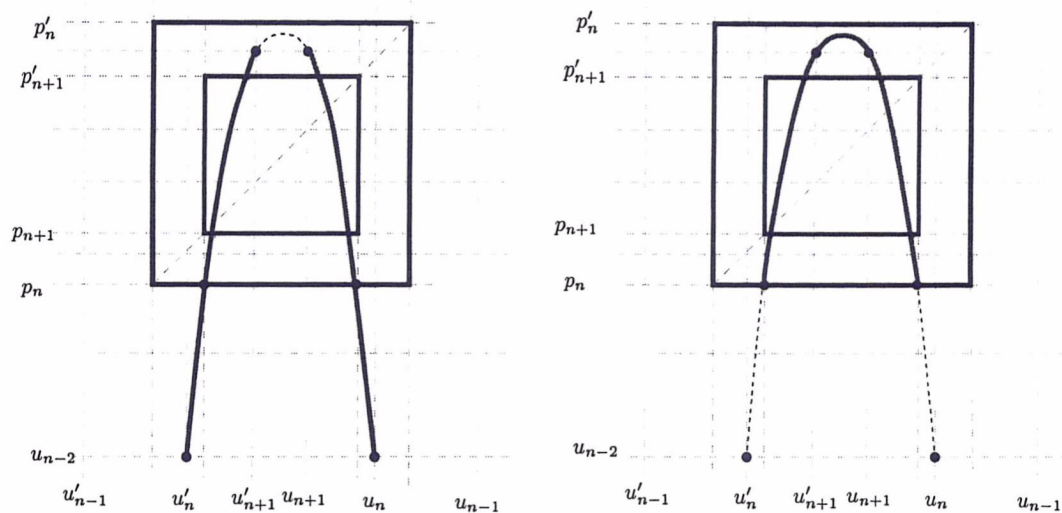
FIG. 3. On the left figure the (green) solid curves represents the part of the f^{S_n} used in the definition of the induced map. On the right figure the (red) solid curve is the part of f^{S_n} which coincides with the n -th Fibonacci renormalization on its central domain.
