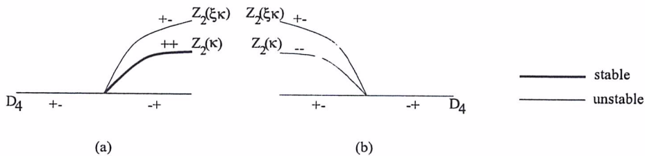
FIG. 6. Bifurcation diagrams for D_4 -reversible-equivariant mappings.
