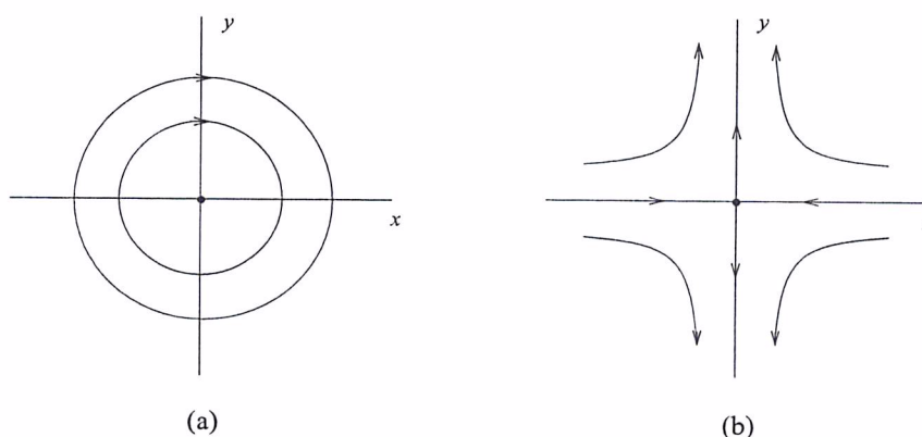
FIG. 1. Schematic phase portraits of two type of flows of vector fields in \mathbb{R}^2 possessing symmetries and reversing symmetries.
