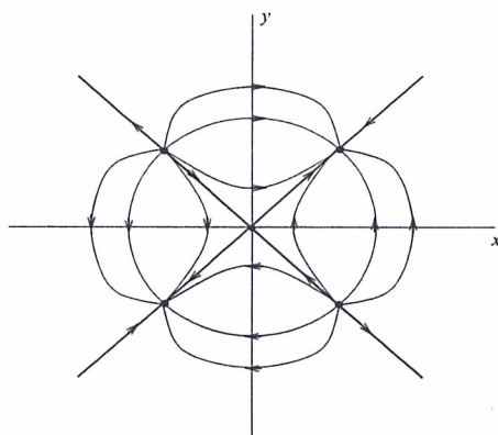
FIG. 2. \mathbf{Z}_4(R) -reversible-equivariant vector field (16) for p(u, v) = q(u, v) = i .
