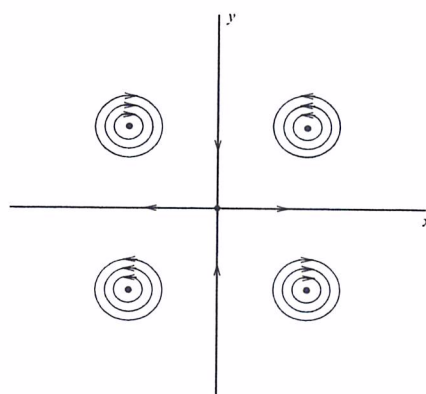
FIG. 5. \mathbf{D}_4(R) -reversible-equivariant vector field (19) for p(u, v) = q(u, v) = 1 .
