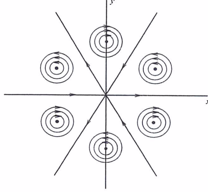
FIG. 4. \mathbf{D}_6(R) -reversible-equivariant (18) vector field.
