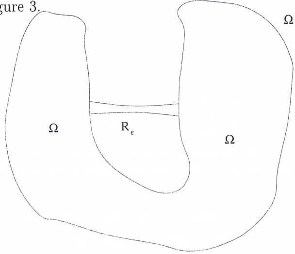
FIGURE 3. Dumbbell domain with a connected \Omega
