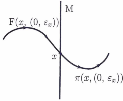
Figure 1: The points of M are isolated in every trajectory of the system (X, \pi) .
