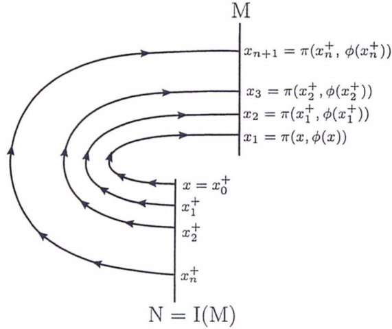
Figure 2: Trajectory in an impulsive semidynamical system (X, \pi; M, I) .
