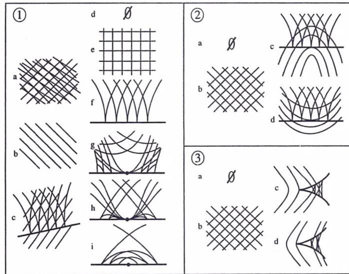
FIGURE 3. Generic configurations of the solutions of an IDE of degree 5 obtained by super-imposing in each quadrant one figure from the left column with one from the right.
