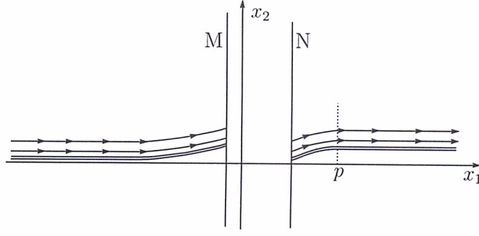
Figure 1: The set A = \{(x_1, x_2) \in \mathbb{R}^2 : x_2 = 0\} is \tilde{\pi} -stable, but it is not uniformly \tilde{\pi} -stable.
