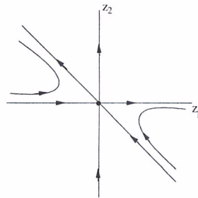
FIGURE 3. The local phase portrait of the vector field (22) and (23) at the origin of chart U_2
