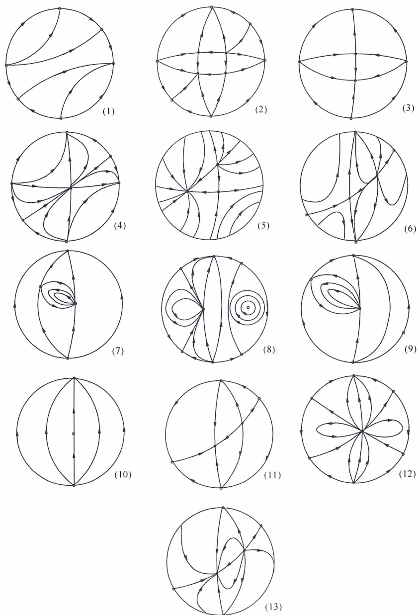
FIGURE 1. The 13 non topologically equivalent phase portraits of the planar quadratic polynomial vector field with a rational first integral of degree 3. The dashed lines denotes lines filled of singular points.
