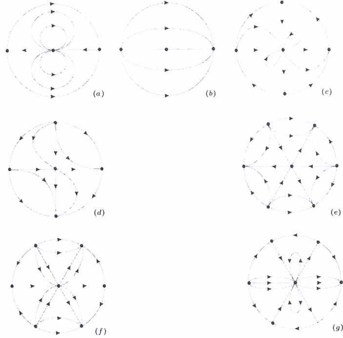
FIGURE 2. The phase portraits of the homogeneous quadratic vector fields.
