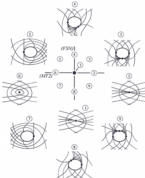
Figure 3: Bifurcations in \mathcal{C}_{\alpha,t} at a D_2^1 umbilic.
