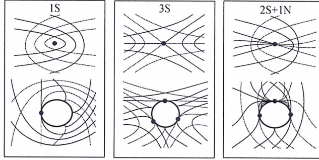
Figure 13: Bifurcations at an A_1^+ Morse Type 2 singularities.
