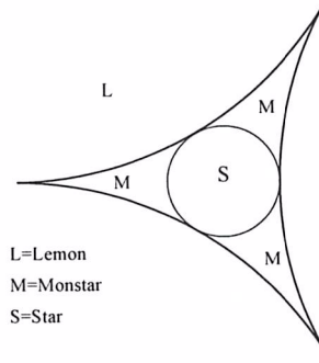
Figure 2: Partition of the \beta -plane.
