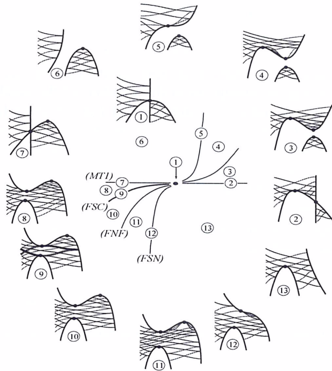
Figure 7: Bifurcations at a non-transverse Morse singularity.
