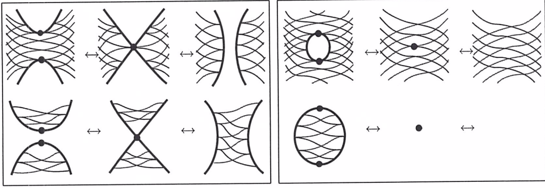
Figure 12: Bifurcations at Morse Type 1 singularities: A_1^- left and A_1^+ right.
