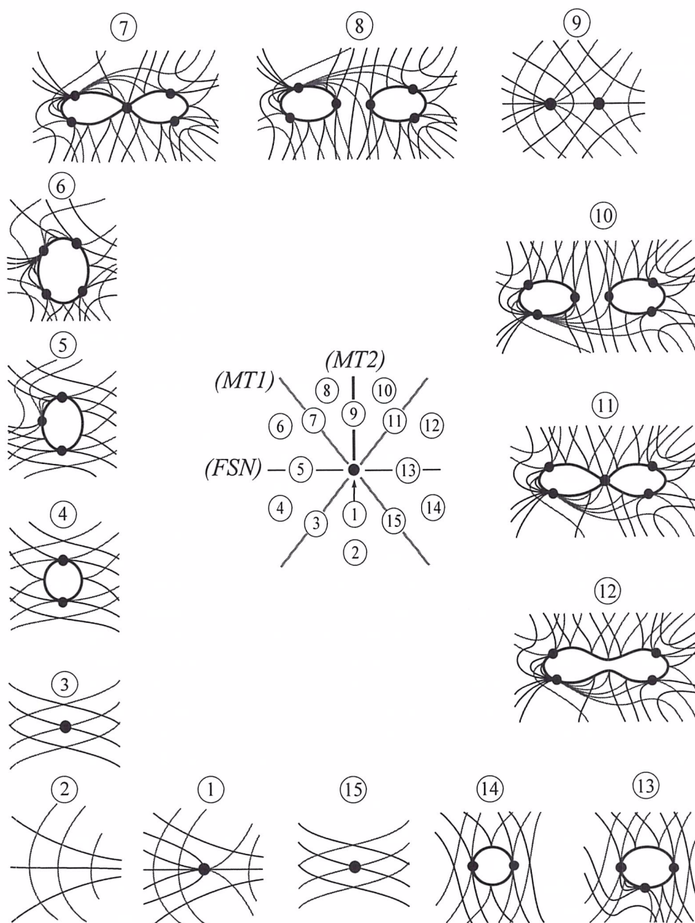
Figure 4: Bifurcations in \mathcal{C}_{\alpha,t} at a D_{2,3}^1 umbilic.
