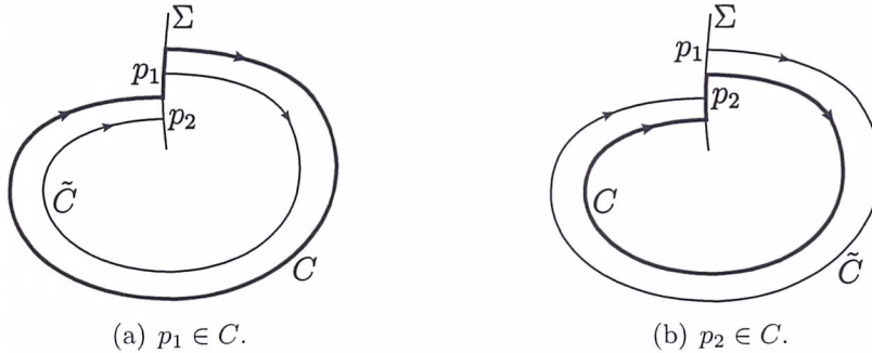
Figure 10: The semi-transversal circles C and \tilde{C} .
