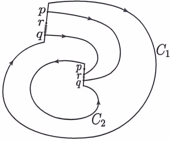
Figure 3: Annulus with boundary C_1 and C_2 .
