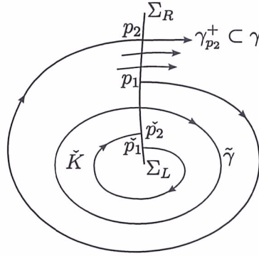
Figure 9: The annulus \check{K} .
