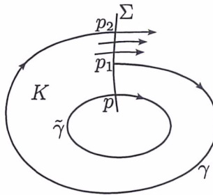
Figure 6: p_1 between p_2 and p .
