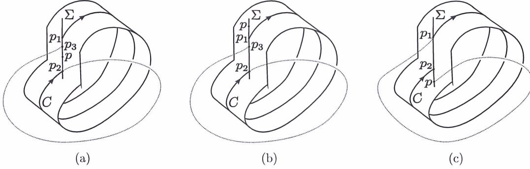
Figure 2: The connectivity of K^2 \setminus C .
