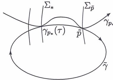
Figure 8: The transversal segments \Sigma_{\tilde{p}} and \Sigma_* .
