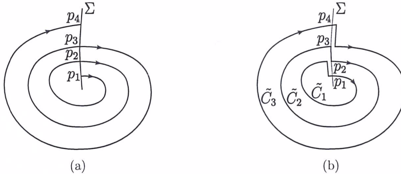
Figure 1: Simple closed curves.
