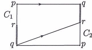
Figure 4: Möbius strip.
