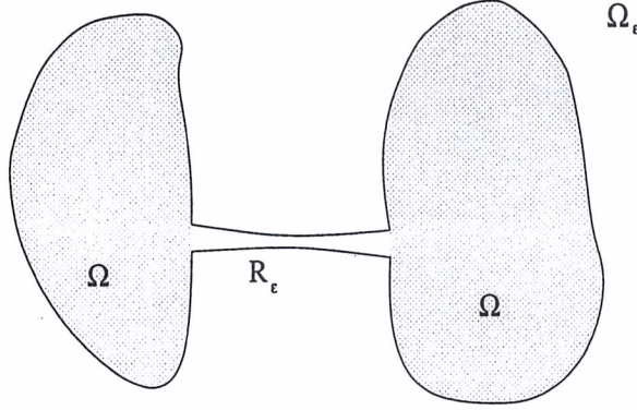
FIGURE 1. Dumbbell domain
