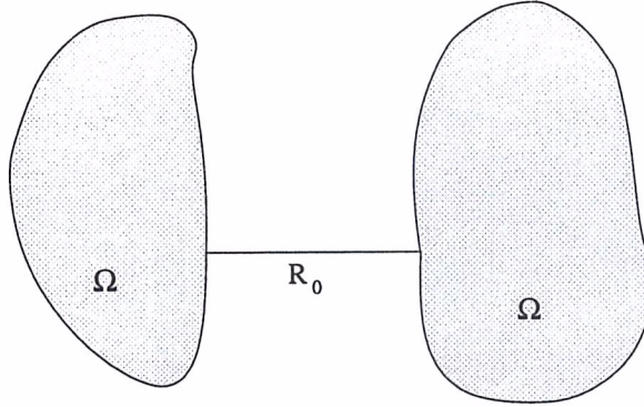
FIGURE 2. Limit "domain"
