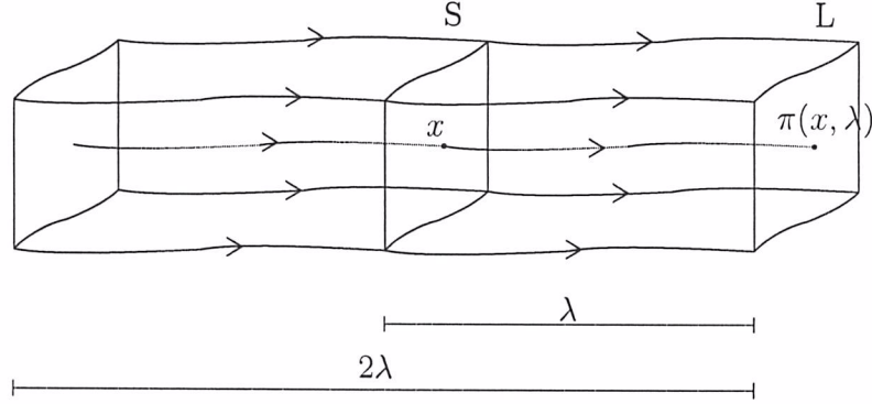
Figure 1: The \lambda -tube F(L, [0, 2\lambda]) .
