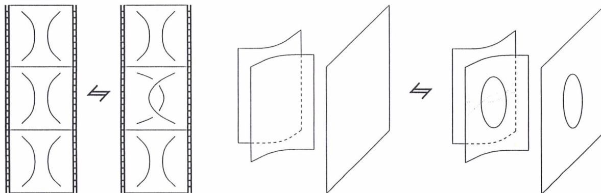
Figure 36: An elliptic confluence of double points
