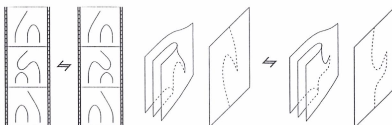
Figure 20: A horizontal cusp
