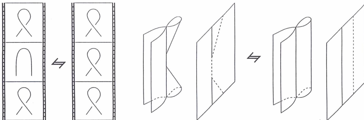
Figure 35: A hyperbolic confluence of branch points
