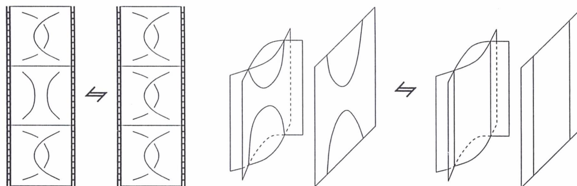
Figure 37: A hyperbolic confluence of double points
