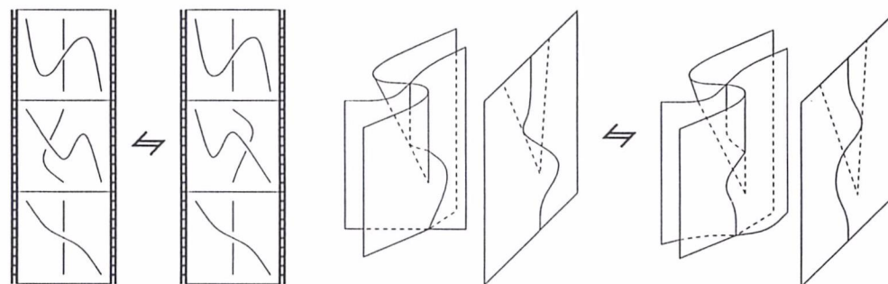
Figure 27: A double arc passes over a fold line near a cusp
