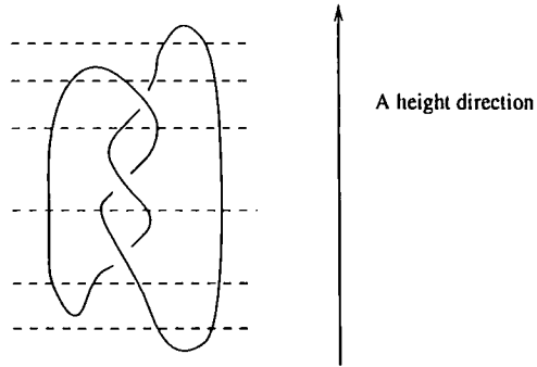
Figure 2: A knot diagram with a height function.
