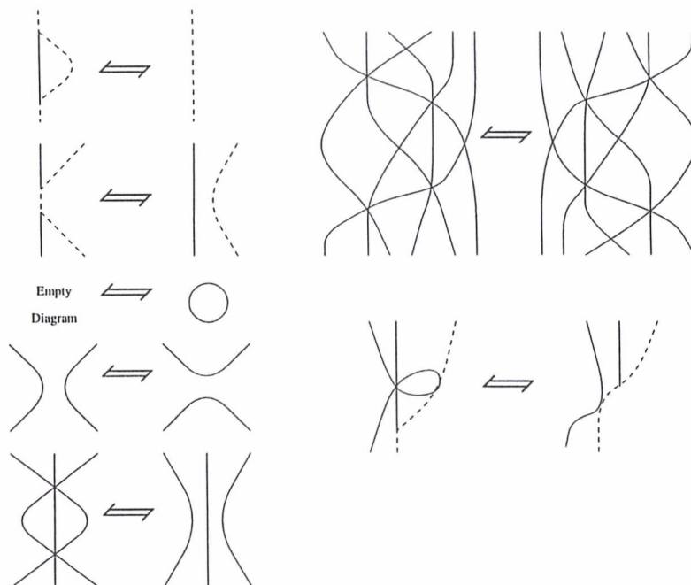
Figure 8: Chart moves, part I
