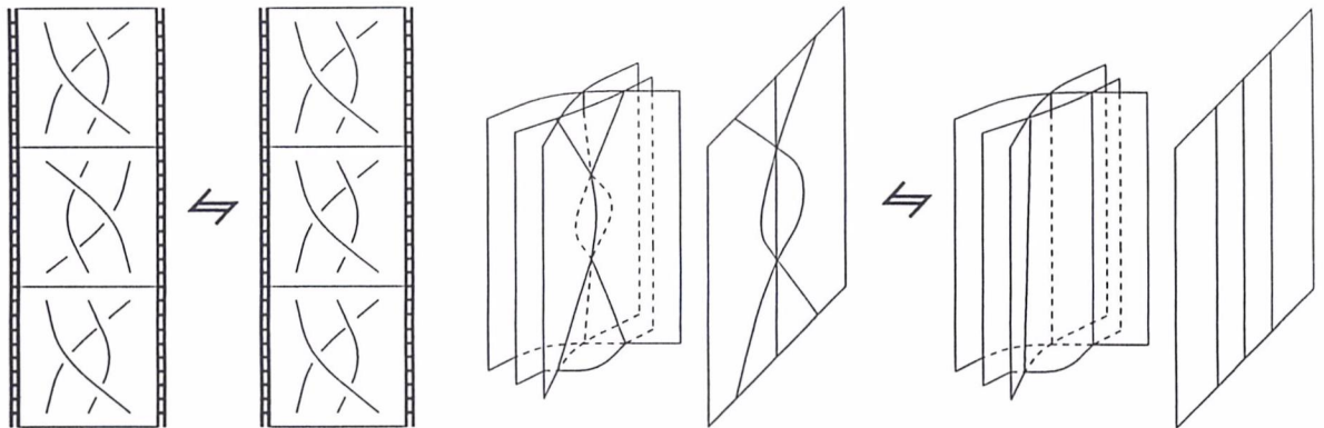
Figure 38: Canceling triple points
