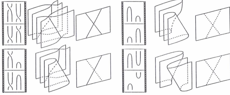
Figure 4: Interchanging crossings and critical points
