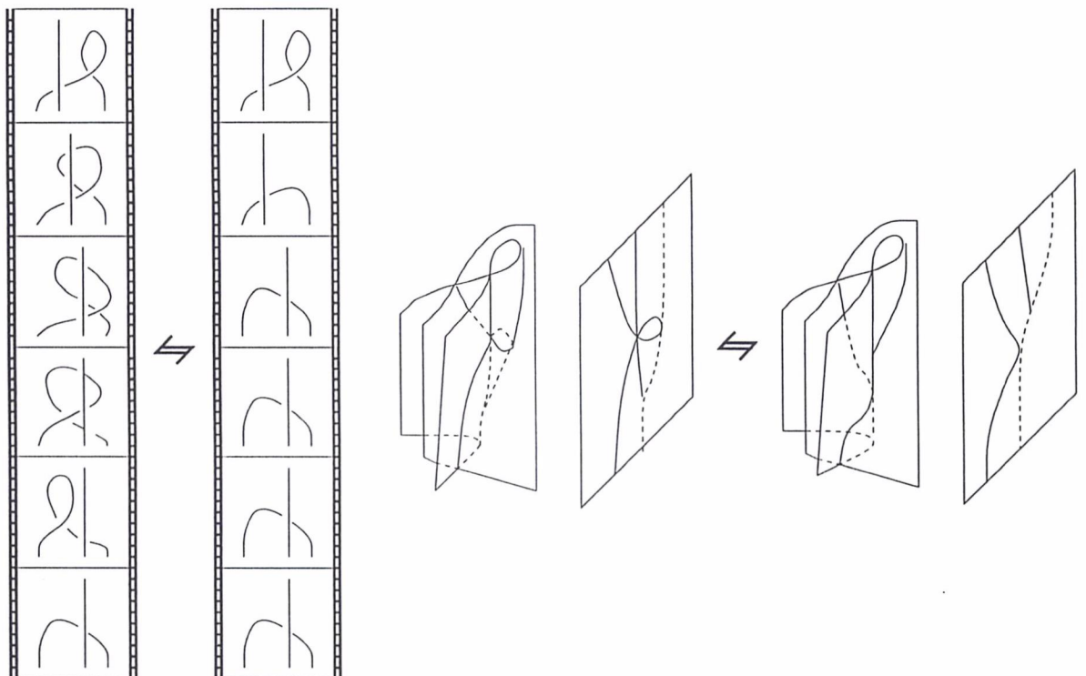
Figure 39: A branch point moving through a triple point
