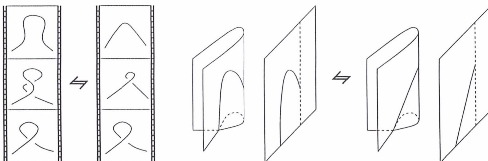
Figure 32: A maximum point of the double point set being pushed through a branch point
