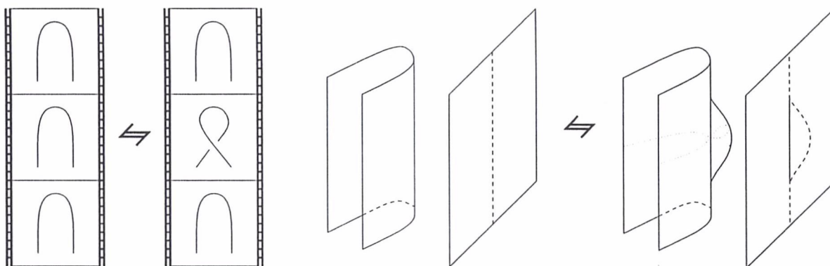
Figure 34: An elliptic confluence of branch points
