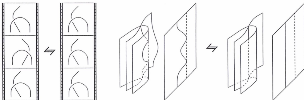
Figure 28: Removing redundant double points crossing the fold lines
