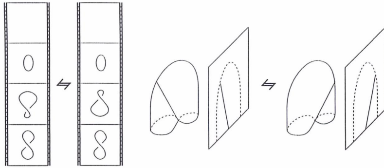
Figure 22: A branch point passes over a maximum point of the surface
