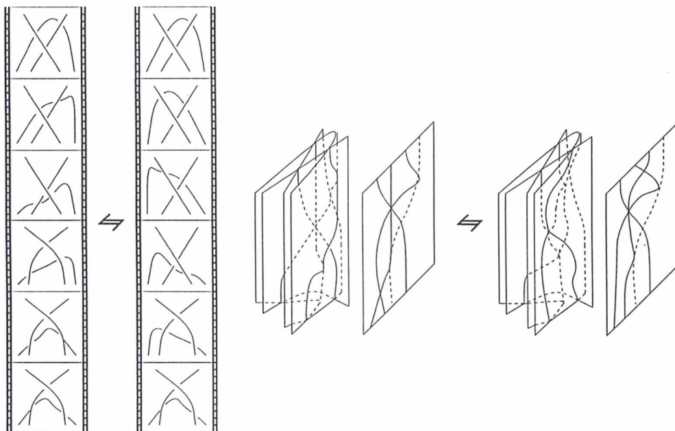
Figure 29: A triple point near a fold line
