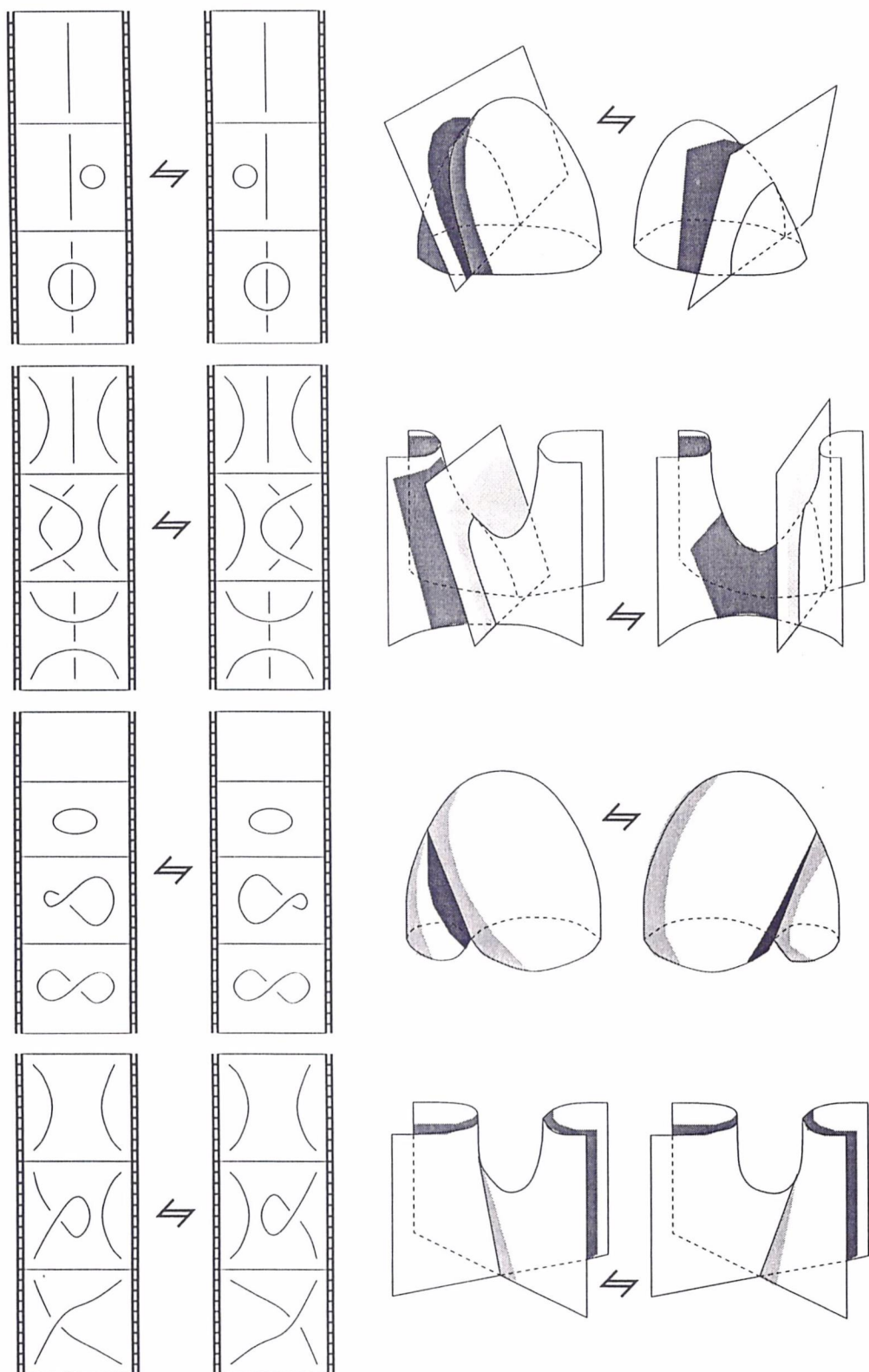
Figure 14: Movie moves in which the topology of the image is unchanged (2)
