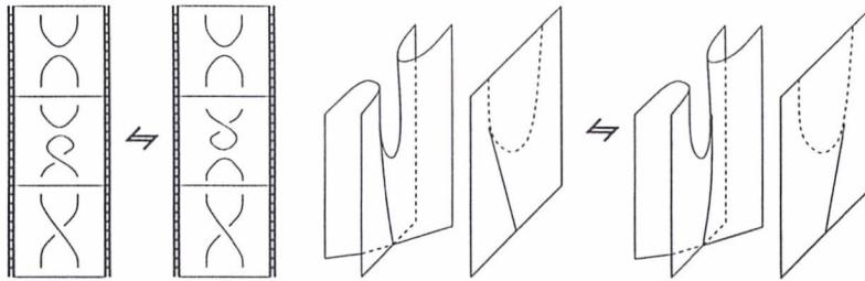
Figure 23: A branch point passes over a saddle point of the surface
