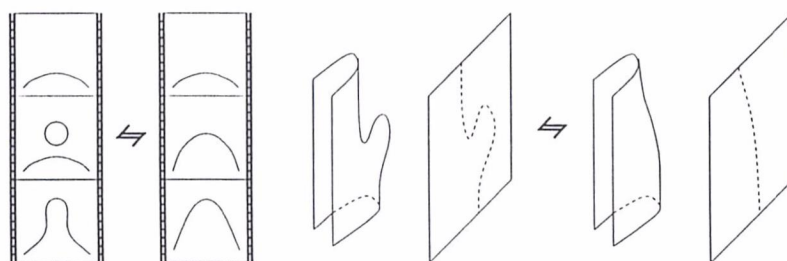
Figure 19: A cusp on the set of fold-lines
