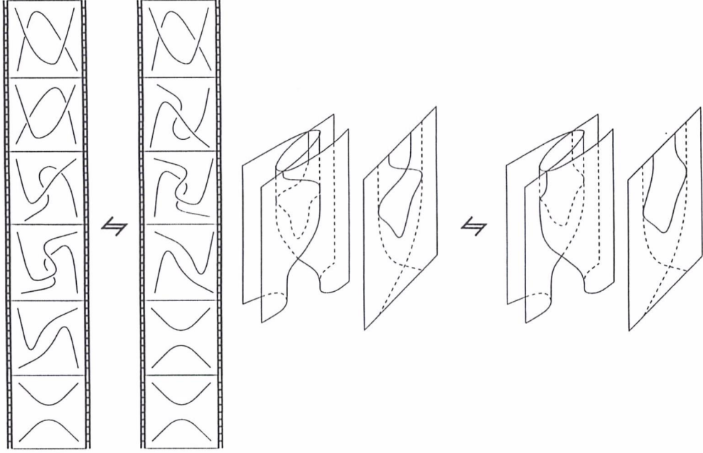
Figure 30: A double point arc becomes tangent to the line of projection
