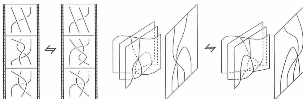
Figure 33: A triple point passing through a maximum on the double point set
