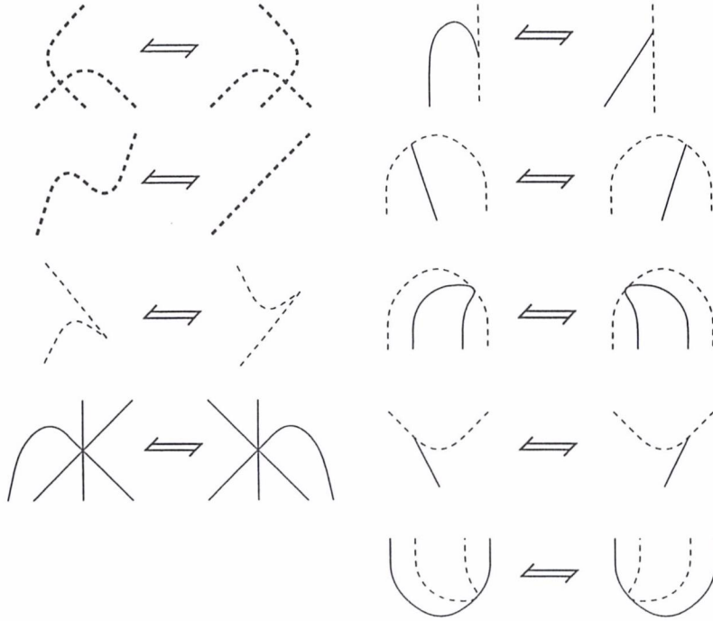
Figure 11: Chart moves, part IV
