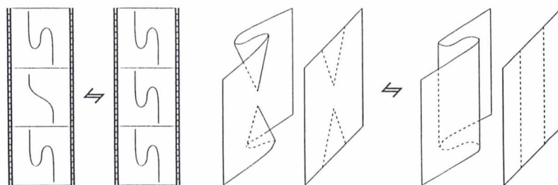
Figure 18: A hyperbolic confluence of cusps
