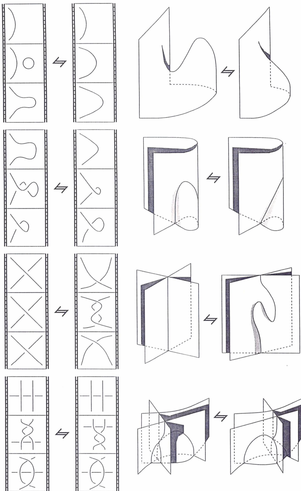
Figure 13: Movie moves in which the topology of the image is unchanged (1)
