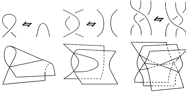
Figure 1: Reidemeister moves and surfaces.
