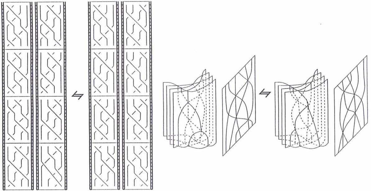
Figure 40: A quadruple point in the isotopy
