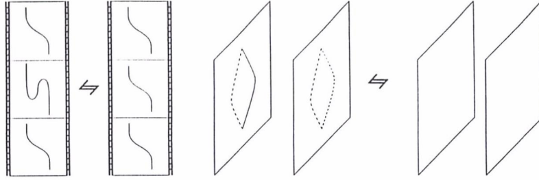
Figure 17: An elliptic confluence of cusps
