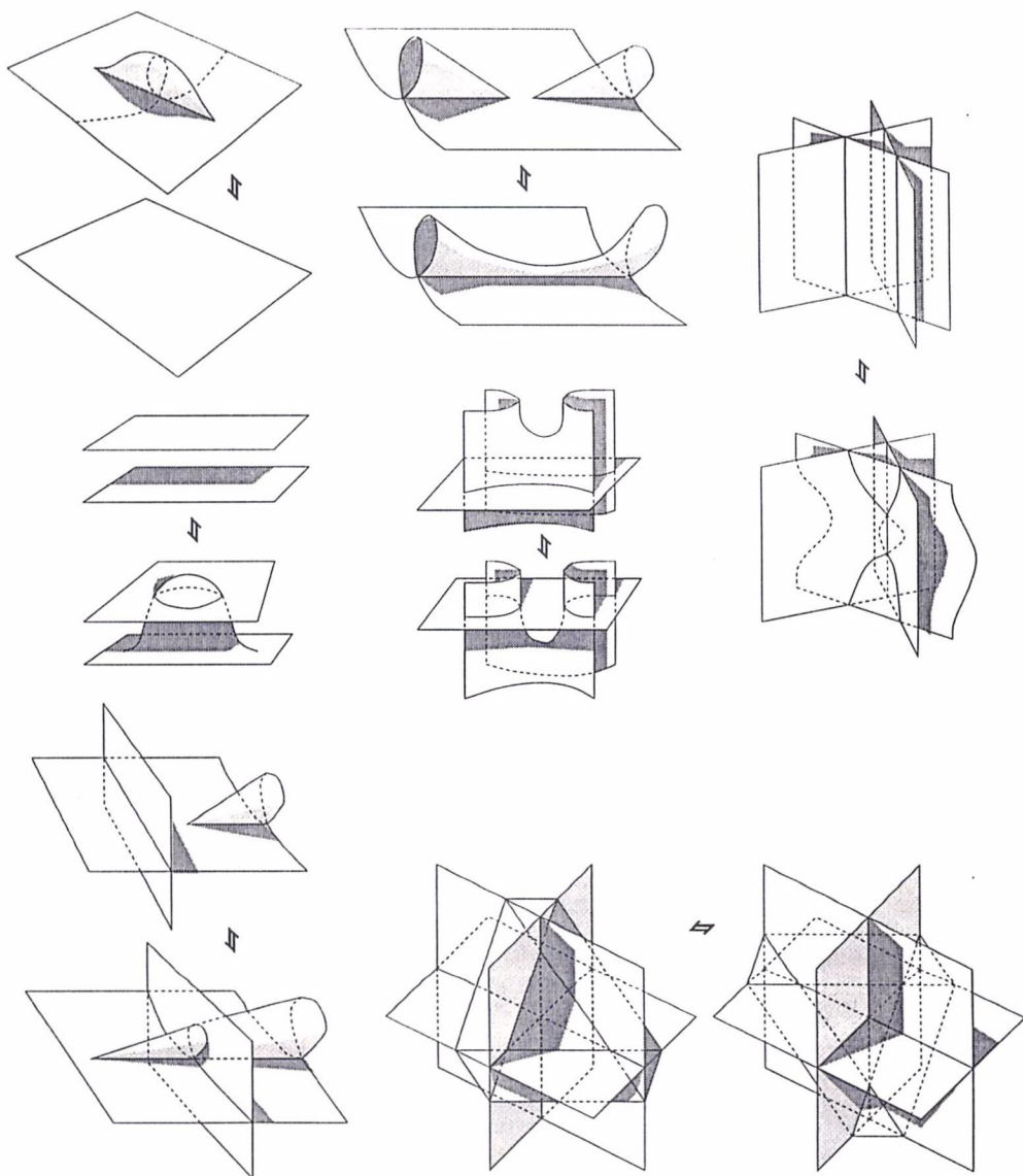
Figure 6: Roseman moves of knotted surfaces
