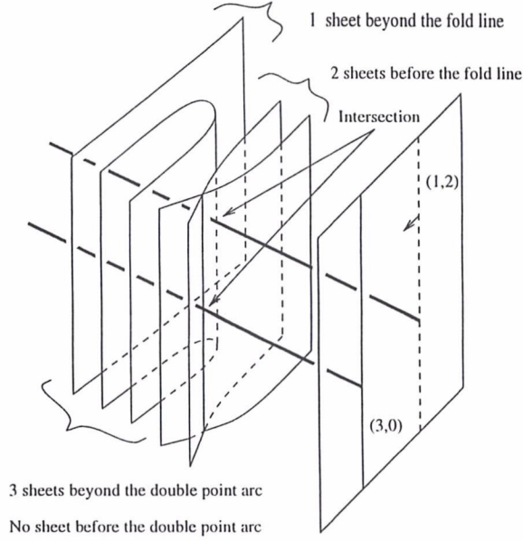
Figure 7: Labeling of charts
