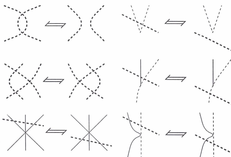
Figure 10: Chart moves, part III
