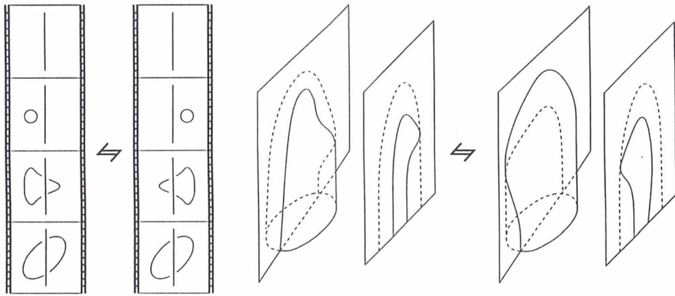
Figure 25: A double point arc passes over a fold line near a maximum point
