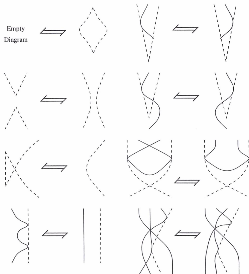
Figure 9: Chart moves, part II
