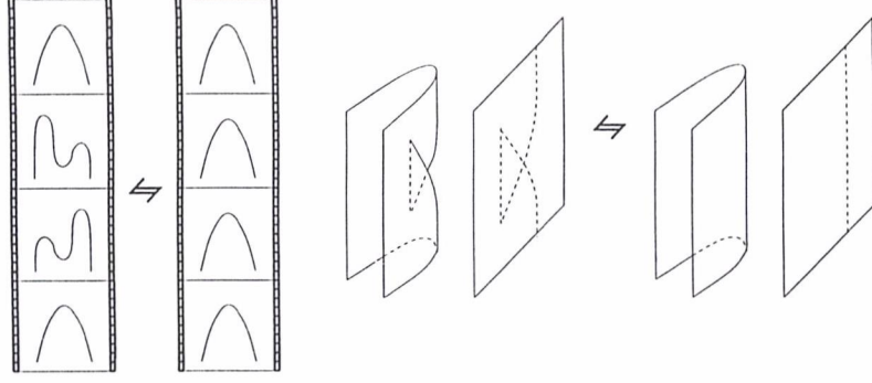
Figure 21: A swallow-tail on the fold lines
