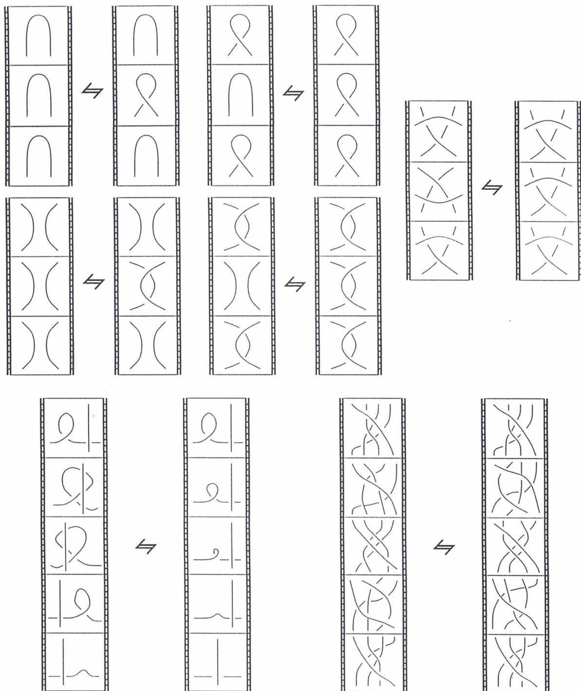
Figure 12: Movie versions of the Roseman moves
