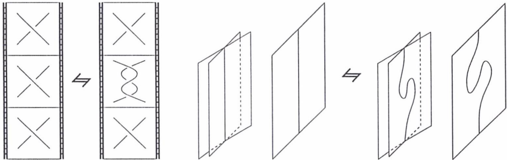
Figure 31: A cusp on the double point set
