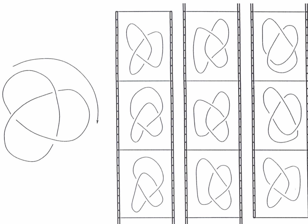
Figure 15: Rotation of trefoil
