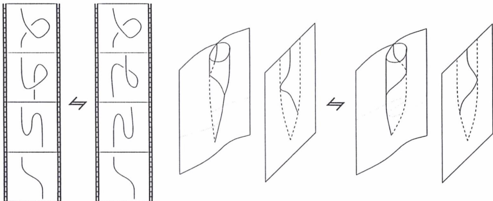
Figure 24: A branch point passes through a cusp
