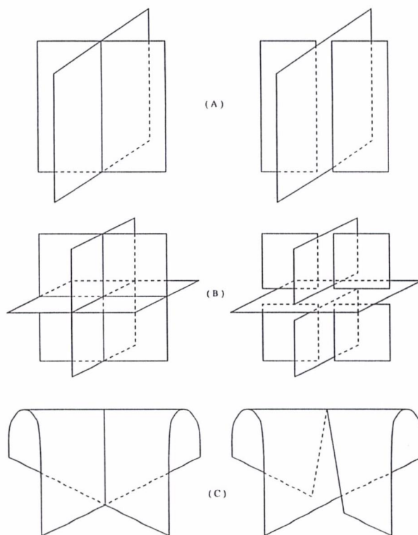
Figure 5: Projections and broken diagrams of knotted surfaces
