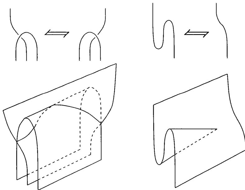
Figure 3: Additional Reidemeister moves with height functions.
