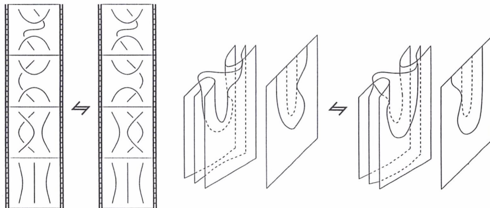
Figure 26: A double point arc passes over a fold line near a saddle point
