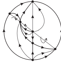
FIGURE 20. The straight line connecting the origin of the local chart U_3 with the singular poin u_1 = u_2 of the local chart U_1 in phase portrait 56 of Figure 18.
