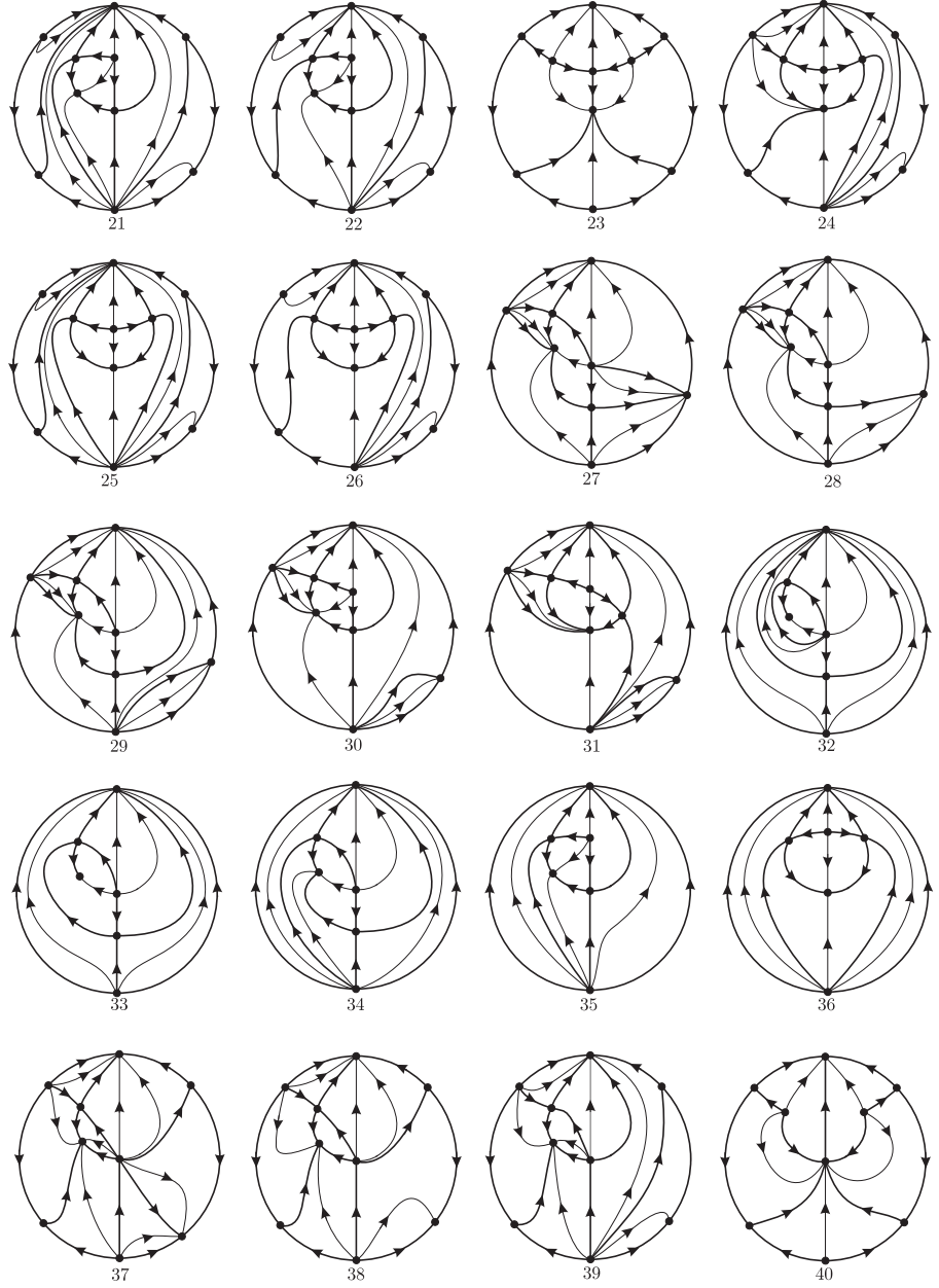
FIGURE 14. Phase portraits of system (P.1) when \gamma_2 = 1 and \beta_2^2 - 4\alpha_2 > 0 .
