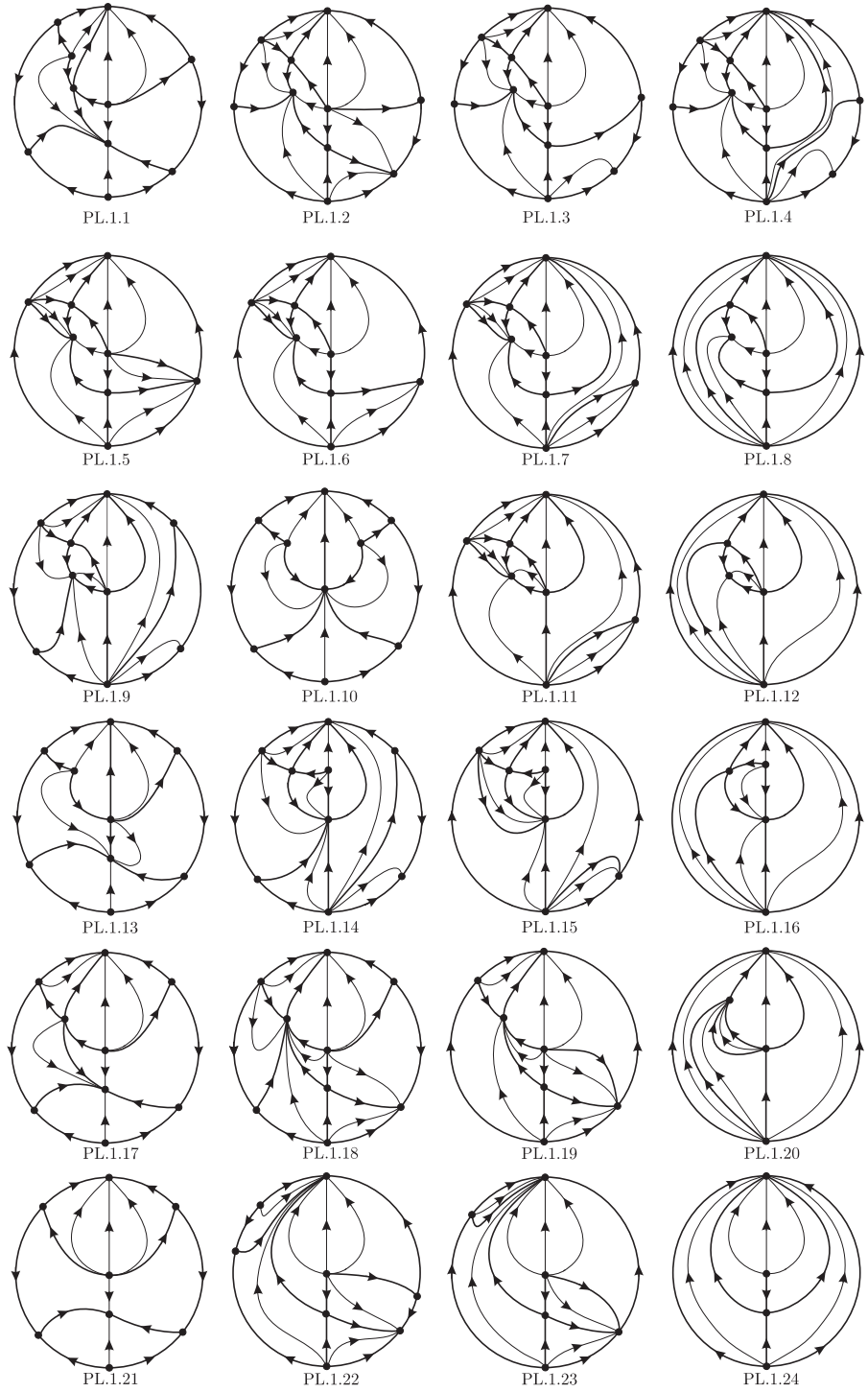
FIGURE 3. Phase portraits of systems of type (P) when they have a Darboux invariant.
