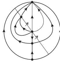
FIGURE 21. The straight line passing through the points z_1 and z_3 in phase portrait 58 of Figure 18.
