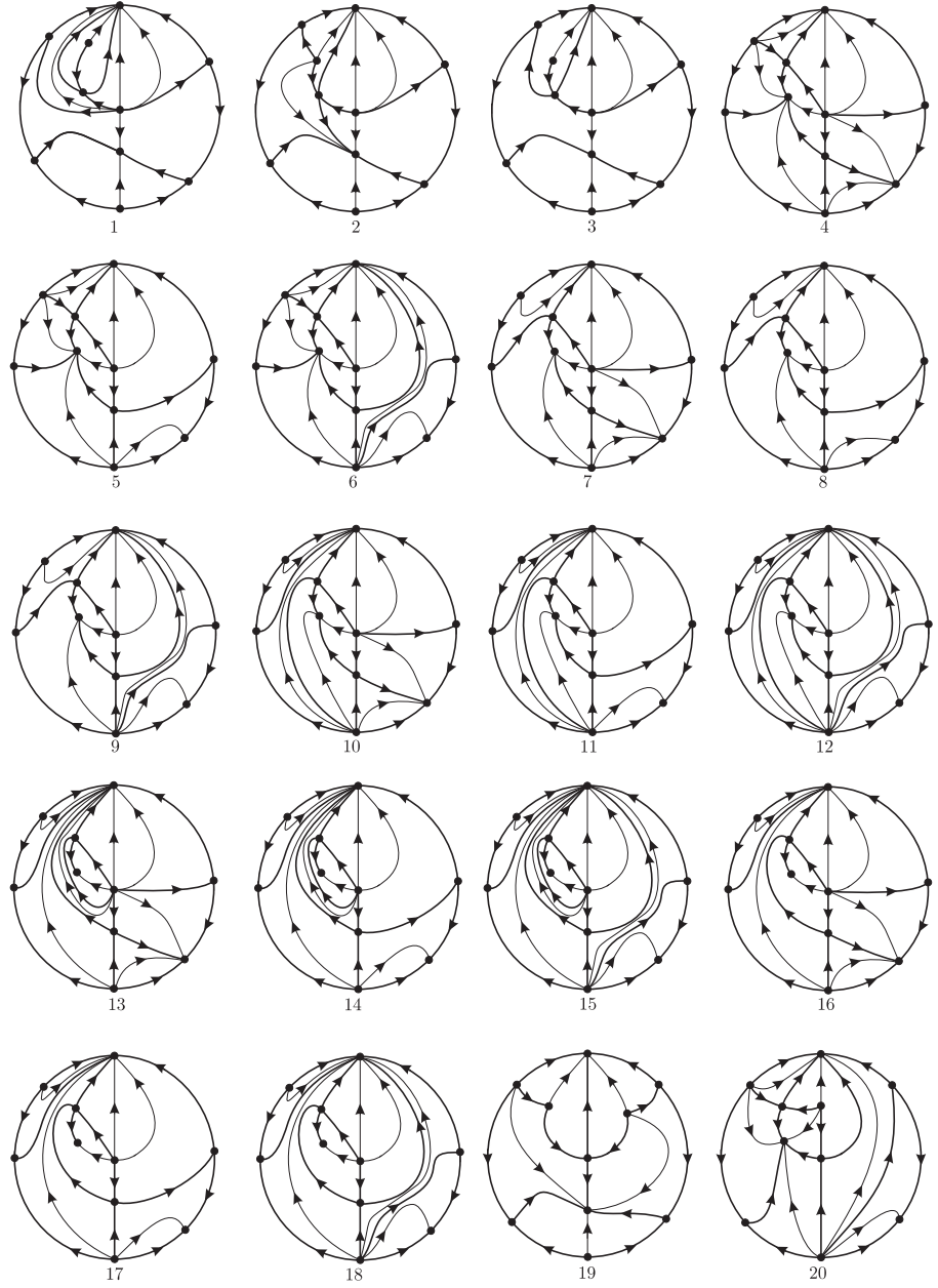
FIGURE 13. Phase portraits of system (P.1) when \gamma_2 = 1 and \beta_2^2 - 4\alpha_2 > 0 .
