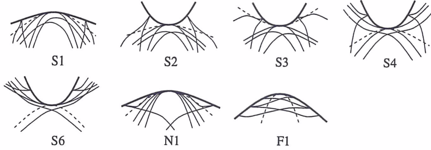
Figure 2: Configurations of asymptotic lines at a cusp of Gauss.
