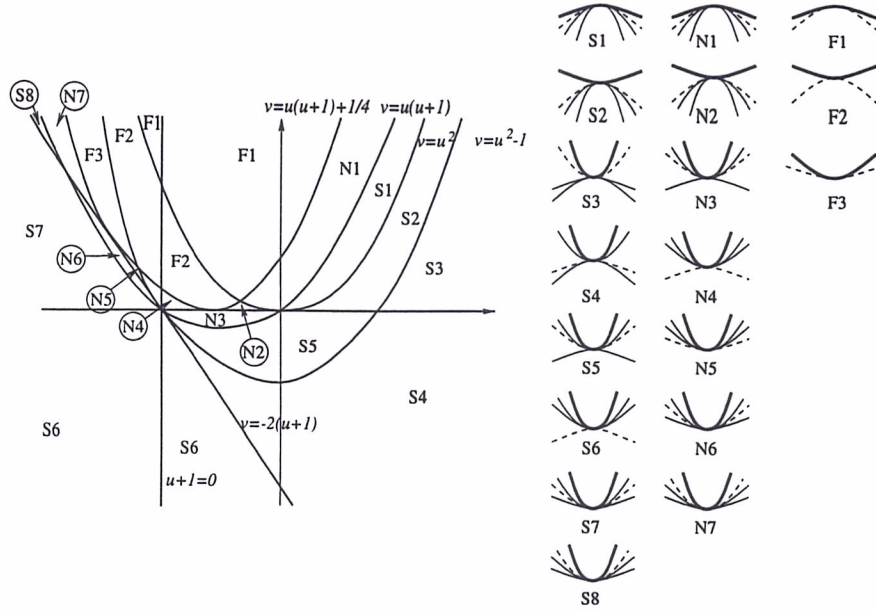
Figure 1: Partition of the (u, v) -plane and the configurations of the cusp set (thick), inflexion set (dashed) and separatrices (thin).
