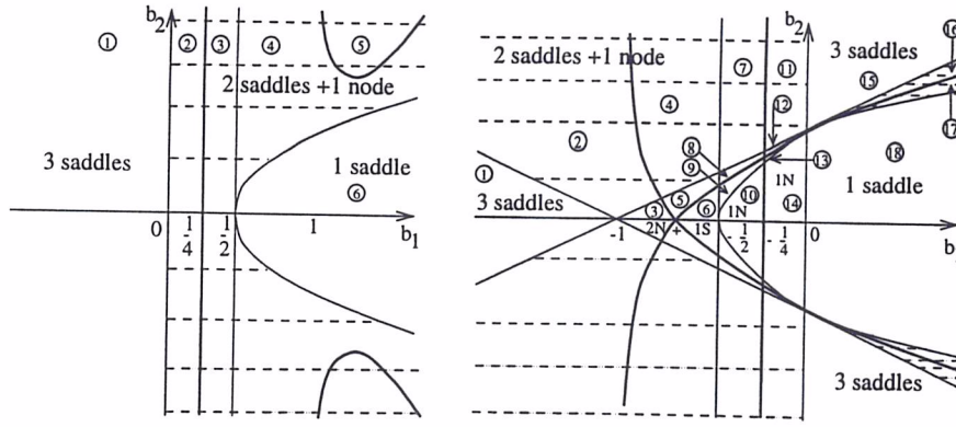
Figure 5: Partition of the (b_1, b_2) plane ( \epsilon = -1 left, \epsilon = +1 right) by the exceptional curves.
