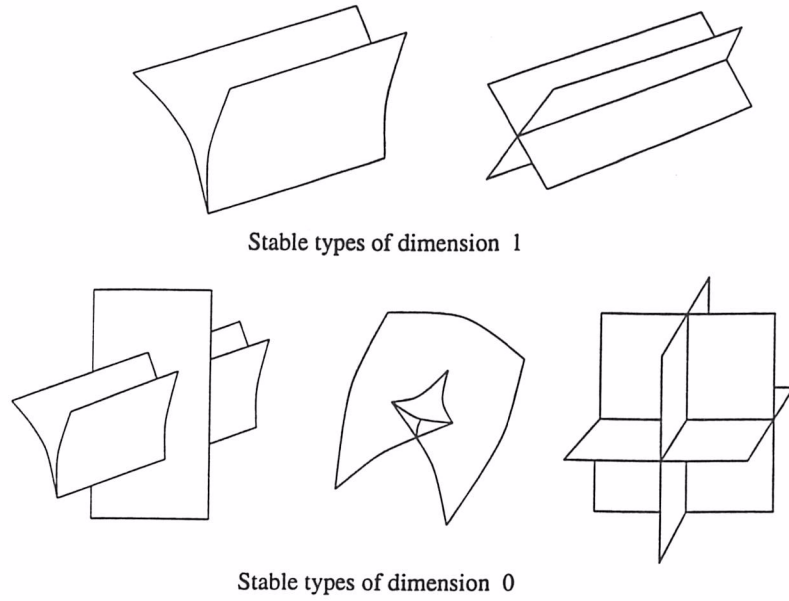
Figure 1: The stable types in the target
